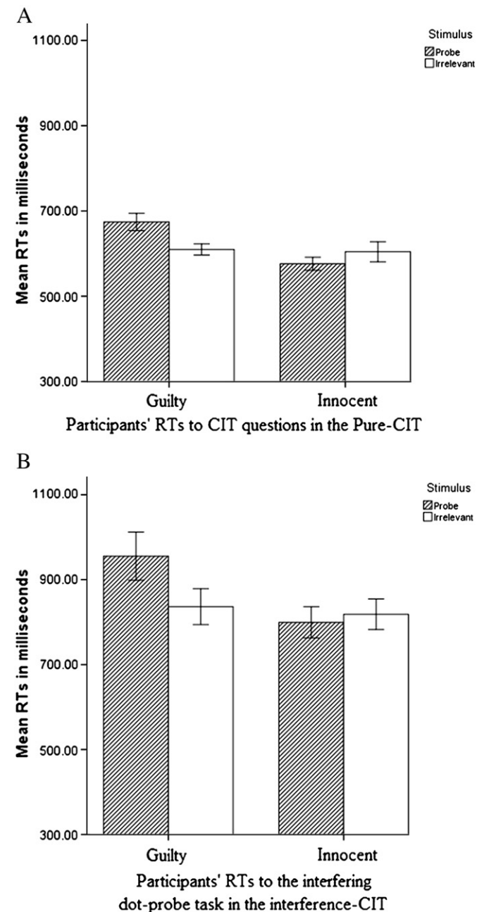
Fig. 2. A: Guilty and innocent participants’ mean of reaction times (RTs) for probe and irrelevant questions in the pure-CIT condition. B: Guilty and innocent participants’ mean RTs for the dot-probe task as a function of probe and irrelevant question type in the interference-CIT condition. The error bar stands for one standard error.
